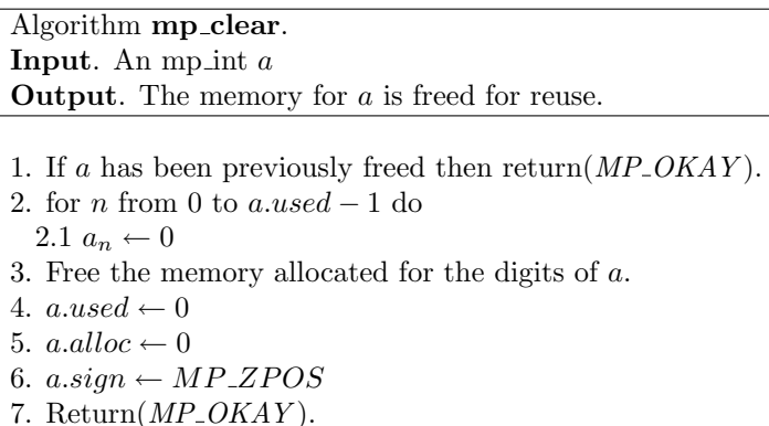
Figure 2.3: Algorithm mp_clear
