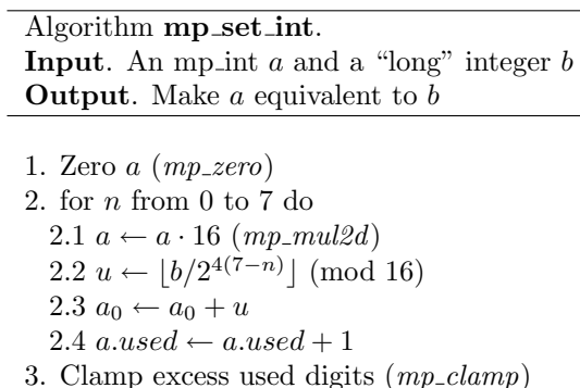
Figure 3.7: Algorithm mp_set_int
