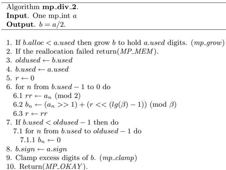
Figure 4.8: Algorithm mp_div_2
