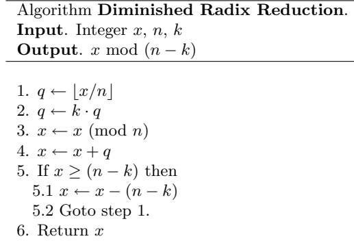
Figure 6.12: Algorithm Diminished Radix Reduction
