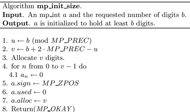
Figure 2.7: Algorithm mp_init_size
